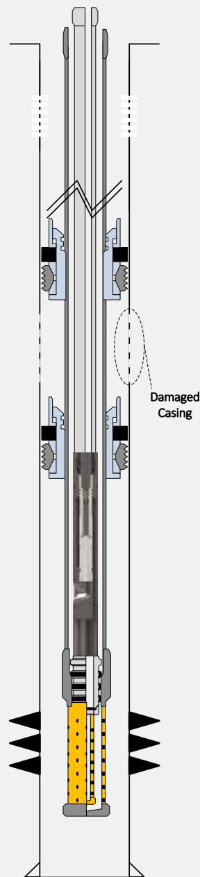
CASING SCAB LINE ISOLATION
